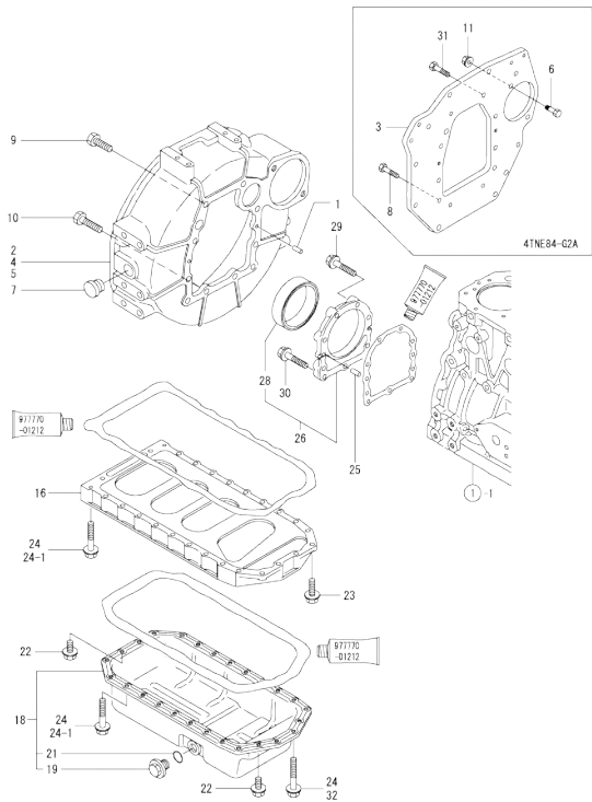
Fig.3. FLYWHEEL HOUSING & OIL SUMP
