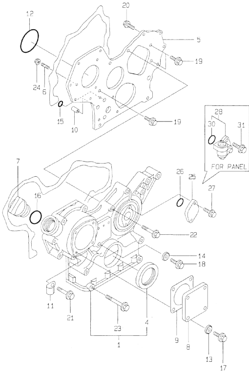
2.GEAR HOUSING
