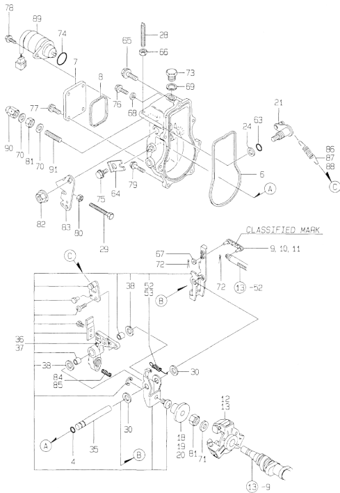
14. GOVERNOR
