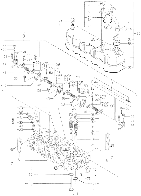
Fig.5. CYLINDER HEAD & BONNET(2)
