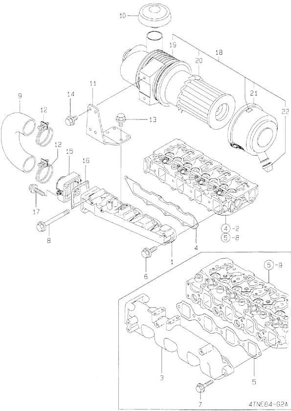
6.SUCTION MANIFOLD & AIR CLEANER
