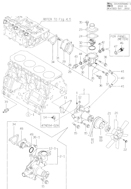
Fig.11. COOLING WATER SYSTEM
