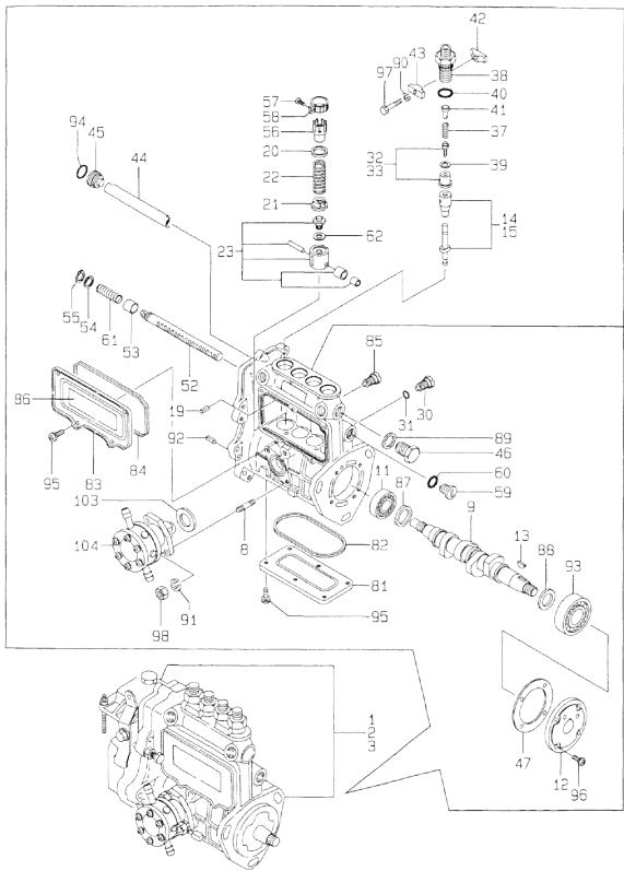
13.FUEL INJECTION PUMP
