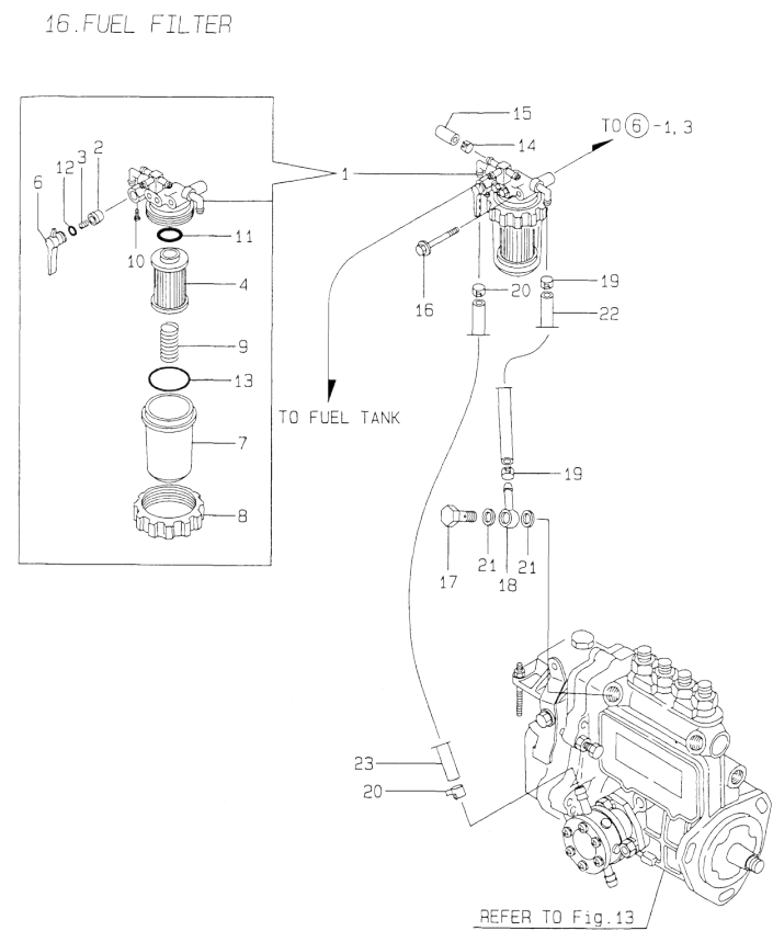
Fig.16. FUEL FILTER
