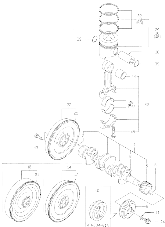
9. CRANKSHAFT & PISTON
