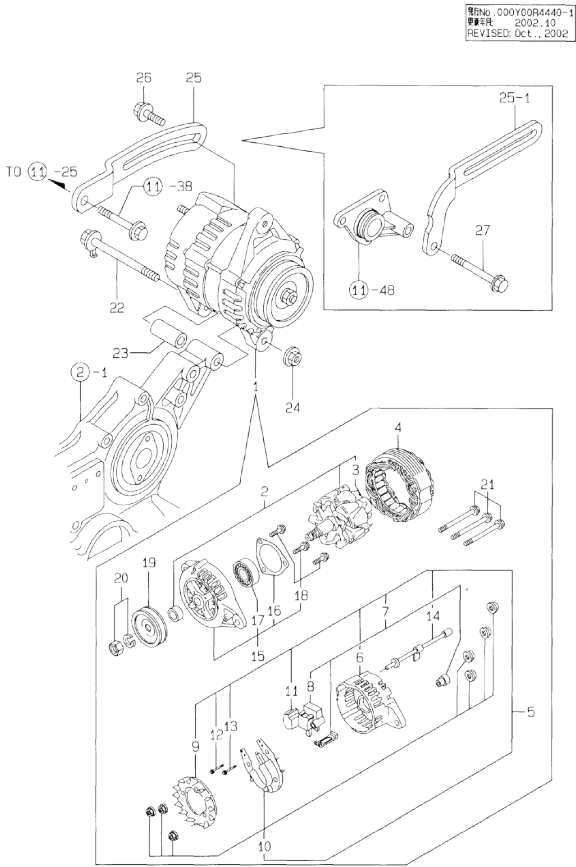
Fig.20. GENERATOR
