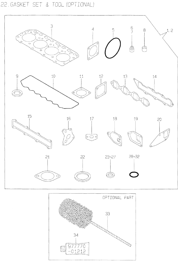
Fig.22. GASKET SET & TOOL(OPTION)
