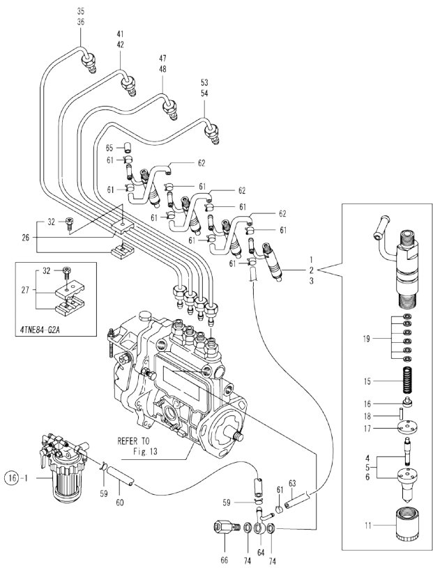
Fig.15. FUEL INJECTION VALVE
